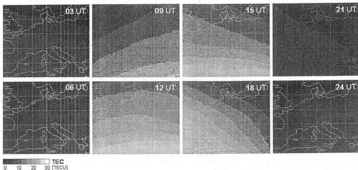
Fig. 10. European TEC forecast (1 hour lead time) based on the NTCM use and the quiet-time geomagnetic activity correction for 3 October 2006 ( 1.0 \leq K_p \leq 2.67 ).
