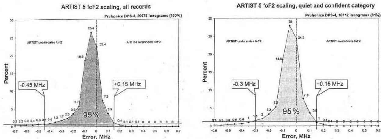
Fig. 1. (Left panel) Error histogram of autoscaled critical frequencies of F_2 layer obtained for 20,675 ionograms from DPS-4 ionosonde at Průhonice, Czech Republic. 95% of all autoscaled values lie within the -0.45 to +0.15 MHz interval from the true values provided by manual scalars. (Right panel) Error histogram for quiet ionospheric conditions and high confidence of autoscaling. Lower bound for foF_2 has improved from -0.45 to -0.3 MHz in comparison to the all ionogram case.
